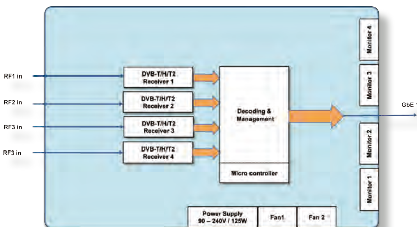
Block Diagram
